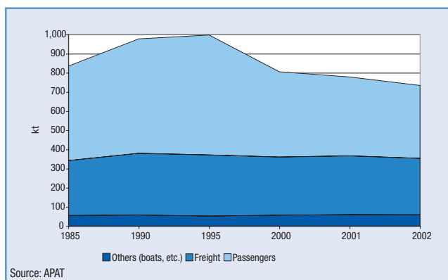
Figure 3.3: Nitrogen oxide emission trend
